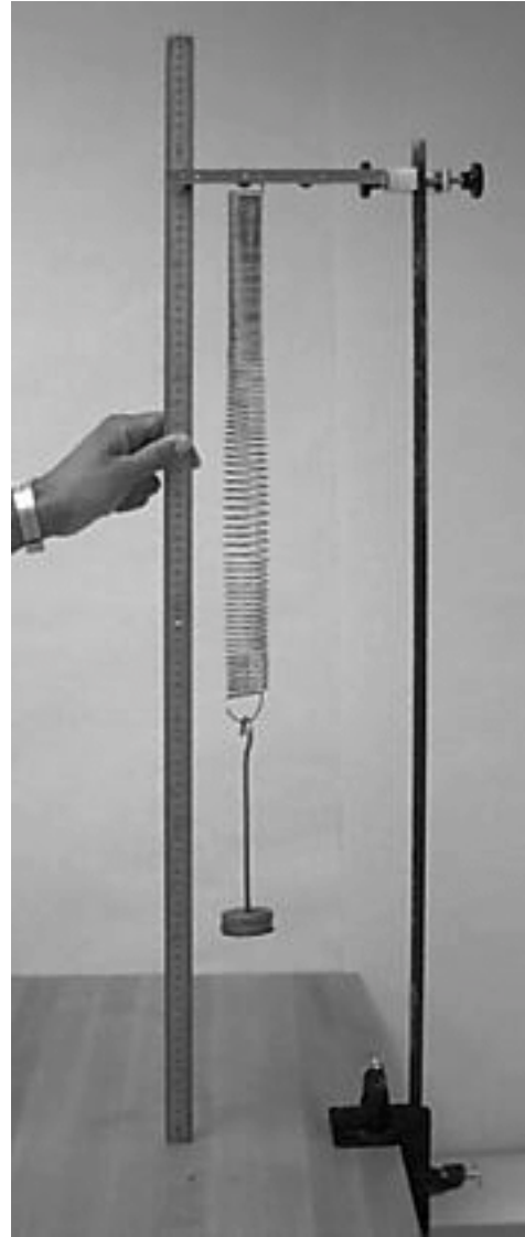
Figure 11-2 Spring-mass oscillator.
