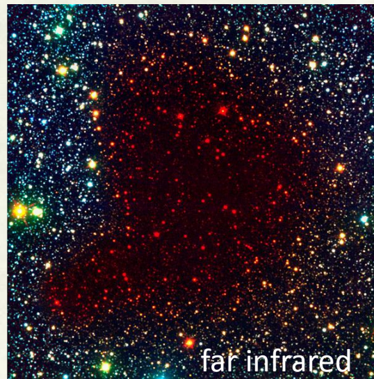
Barnard 68 dark nebula (dust cloud)
